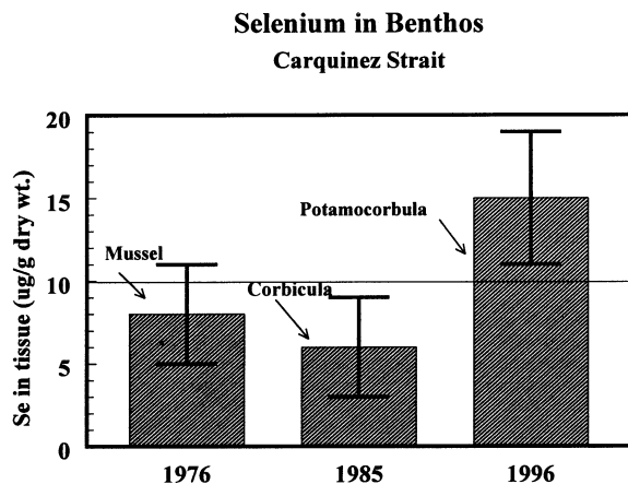
Fig. 6. Mean and S.D. of Se concentrations ( \mu\text{g Se per g dw} ) in three studies of bivalves from in or near Carquinez Strait in three different decades. 'Mussels' were studies of transplanted M. edulis in 1976 (Risebrough et al., 1977); 'Corbicula' represents mean of 67 samplings of the clam C. fluminea (Johns et al., 1988) and 'Potamocorbula' is the mean of all Carquinez samples in the present study.
