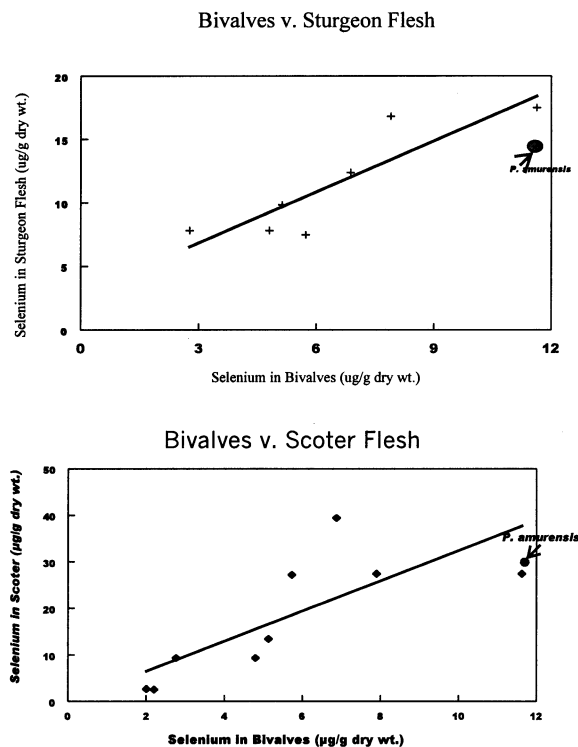
Fig. 7. Relationships between Se concentrations in resident bivalves (data from White et al., 1988; Urquhart and Regalado, 1991; Johns et al., 1988) and either sturgeon flesh or the flesh of the diving ducks (surf scoter) from North San Francisco Bay and Humboldt Bay (data from White et al., 1987, 1988, 1989; Urquhart and Regalado, 1991). Predators and prey were sampled in the same season, year and sub-bay. Mean Se concentration in P. amurensis at Carquinez in 1995 is superimposed on each graph to match predator data from 1989–1990, because P. amurensis was probably the primary food of these predators in 1989–1990.
